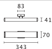
Z640RS Vanity 16 W
