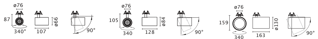
Z235CC Track empotrar 10 W
